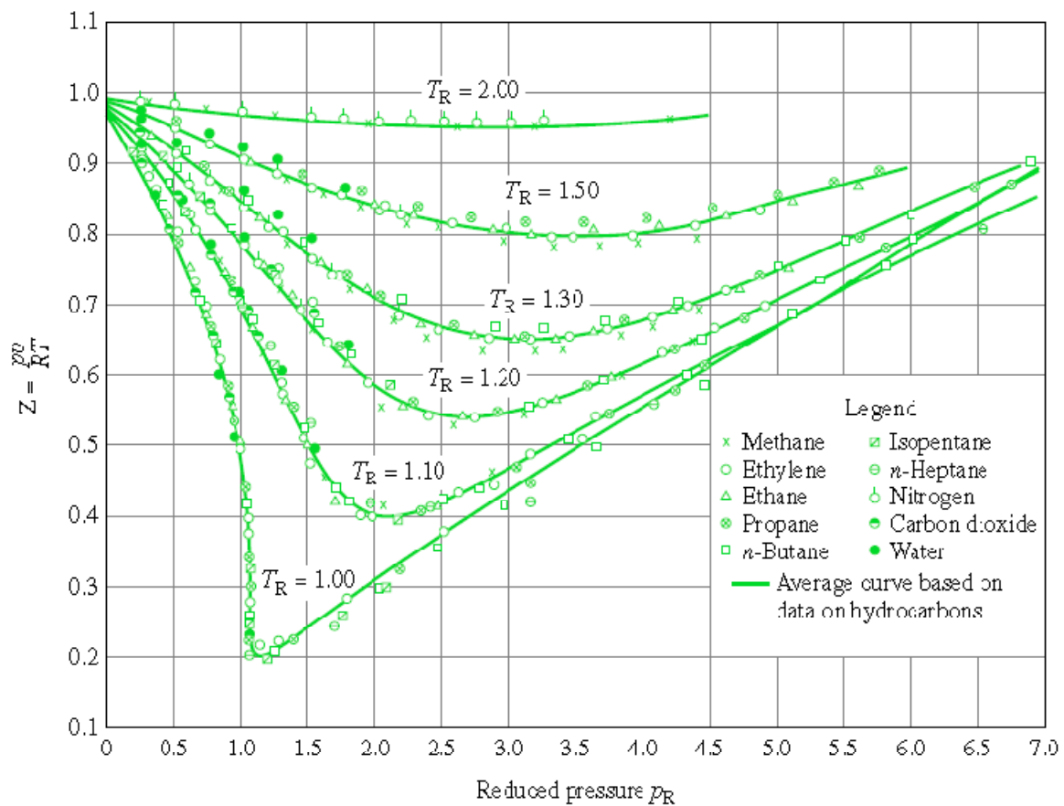
▲ Figure 3.12 Generalized compressibility chart for various gases.
